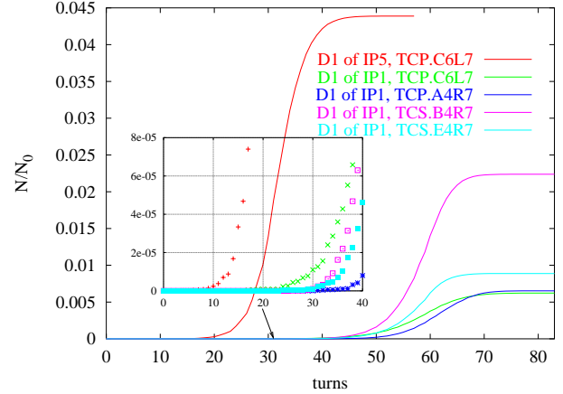
Figure 3: Number of particles hitting the collimators in IR7 relative to the initial number N_0 for a powering failure of the D1 magnets. Particles in the core of the bunch were not tracked.
