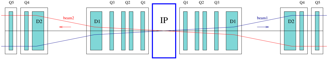
Figure 2: Illustration of the magnet placing at the interaction point
