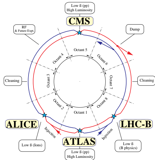
Figure 1: Layout of the LHC
