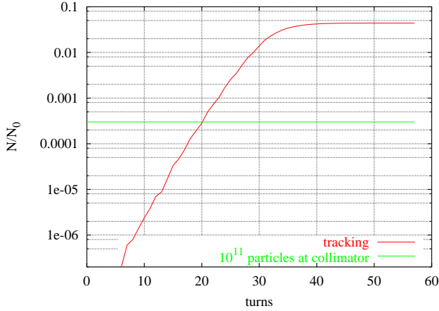
Figure 4: Power converter failure at the D1 magnets in IP5. Particles in the core of the bunch were not tracked.
